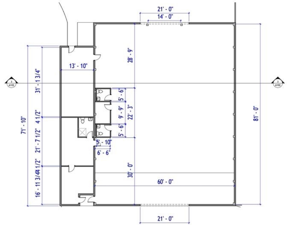
2 First Floor Architectural Plan 1/8" = 1'-0"
