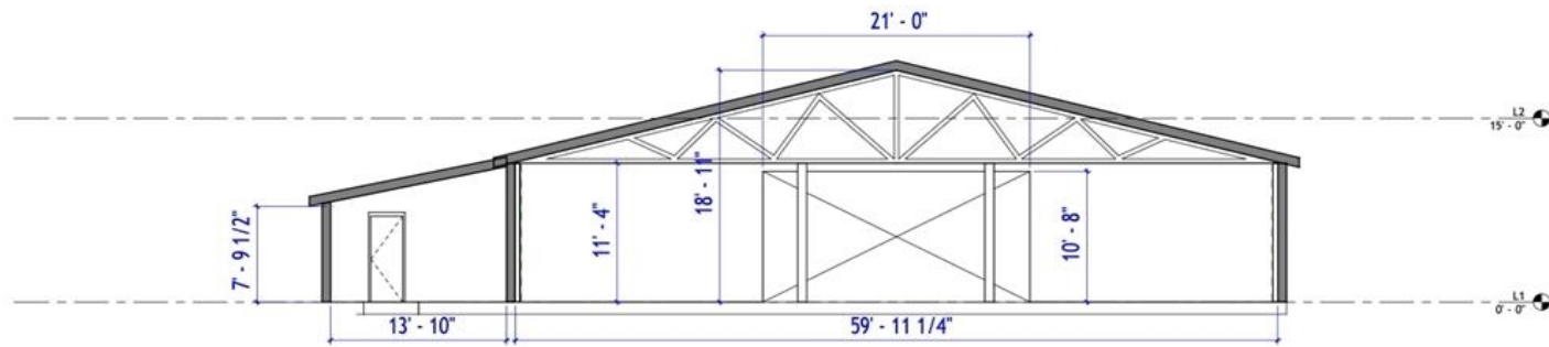
3 Section 1 3/16" = 1'-0"
